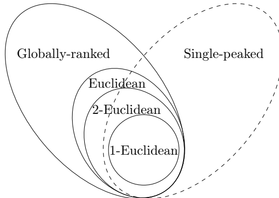
Figure 1: Relationships between globally-ranked, single-peaked, and Euclidean preference domains.
