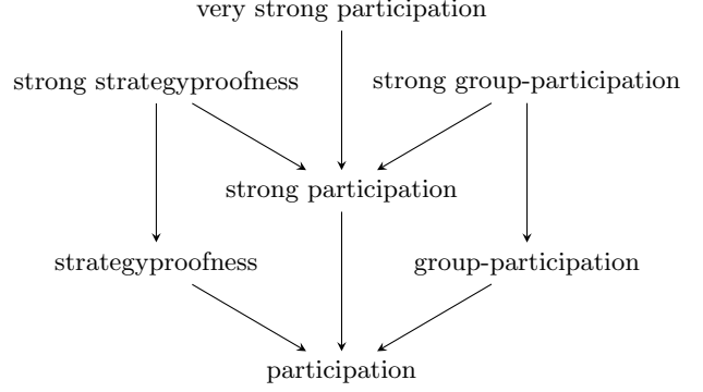
Figure 1: Implications between the different notions of participation and strategyproofness. An arrow from one notion to another signifies the former implies the latter.
