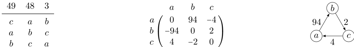
Figure 1: Illustration of the definitions given in Section 2. The table on the left represents a preference profile R for three alternatives a, b, c and 100 voters. The number on top of each column denotes the number of voters with the corresponding preference relation, e.g., there are 49 voters with the preference relation \succsim_i: c, a, b . The corresponding matrix of majority margins and the weighted digraph are displayed on the right. The majority relation of R is cyclic, i.e., a \succ_R b \succ_R c \succ_R a . Hence, R does not admit a (weak) Condorcet winner.
