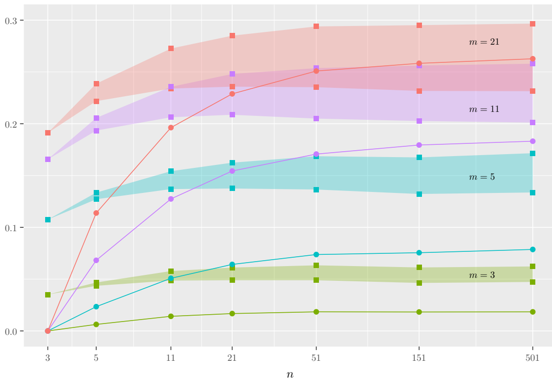
Figure 8: Average normalized Shannon entropies of ML schemes with the lower boundary of each colored area corresponding to C2-ML and the upper boundary corresponding to C1-ML . Additionally, the average distances between these two ML schemes according to the L^1 -norm are displayed as solid lines. The same set of sampled profiles as in Figure 7 is used.
