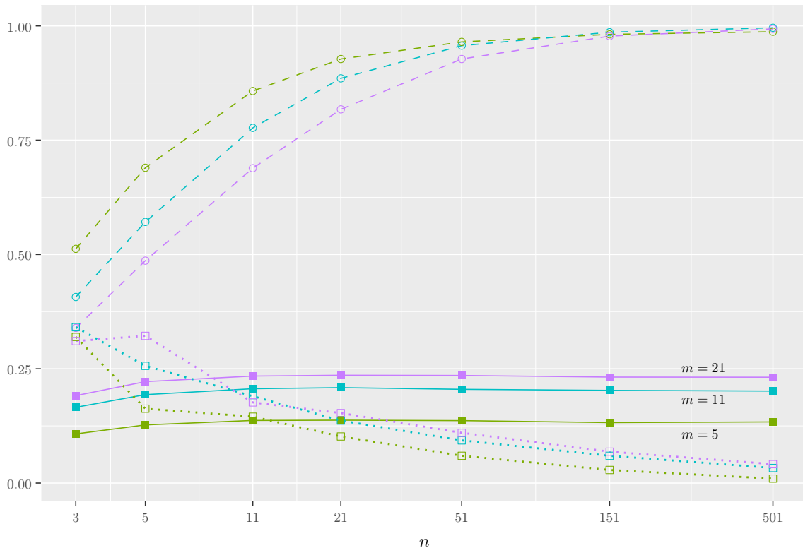
Figure 9: Average normalized Shannon entropies of C2\text{-ML} (solid line) compared to random dictatorship (dashed line) and the plurality rule (dotted line). For C2\text{-ML} the same set of sampled profiles as in Figure 7 is used.
