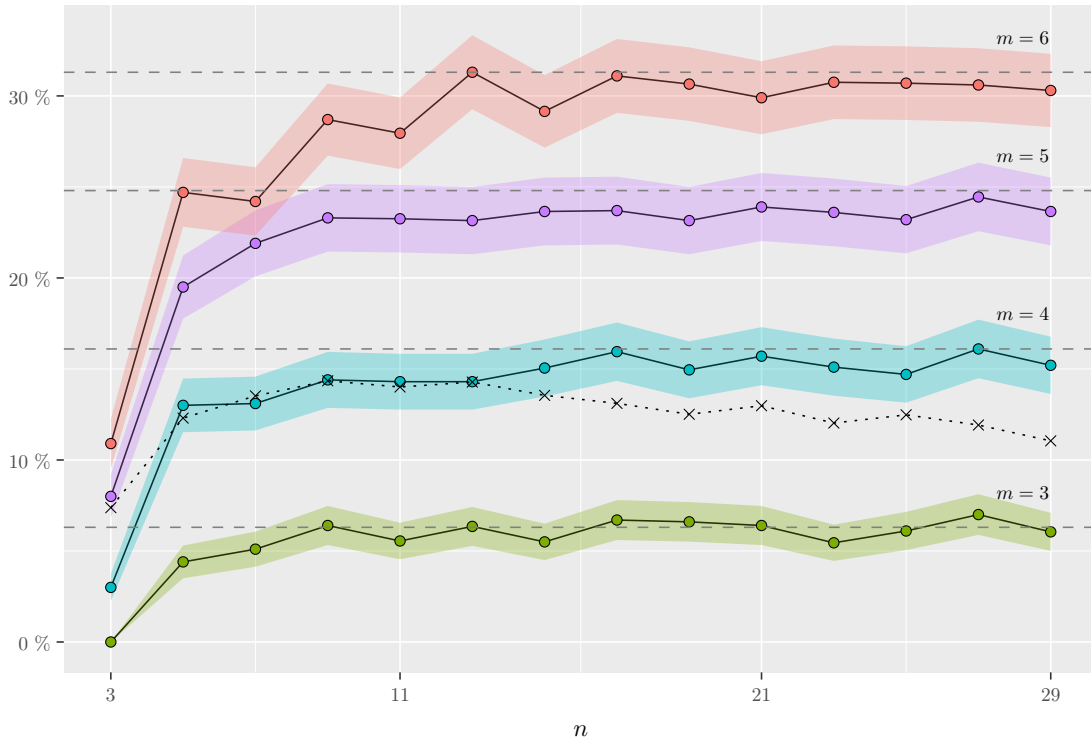
Figure 10: SD -manipulability of C2-ML (solid lines) with confidence intervals for a confidence level of 95% (in color) and manipulability of C1-ML for m = 5 (dotted line). Each point is based on 2000 preference profiles sampled according to the IAC model and on testing all possible deviations for each type of voter. The dashed lines show the limit probabilities that no Condorcet winner exists for n \rightarrow \infty derived by Gehrlein (2002).
