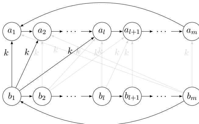
Figure 3: Weighted majority graph for which the support of the unique lotteries returned by ML^\tau and ML^\sigma have disjoint supports. All unlabeled edges have weight 1. Missing edges point downwards with weight 1.
