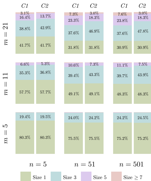
Figure 7: Distributions of the support sizes of C1 -ML (left) and C2 -ML (right) for m \in \{5, 11, 21\} and n \in \{5, 51, 501\} for 100.000 samples for every combination of parameters according to the IAC model. The bars represent the frequency of a support with size 1, 3, 5, and 7 or more stacked from bottom to top. Frequencies lower than 3% are not labeled.
