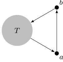
Figure 1: Tournament C(T, I_a, I_b) for a given tournament T . The gray circle represents a component isomorphic to the original tournament T . An edge incident to a component signifies that there is an edge of the same direction incident to each alternative in the component.
