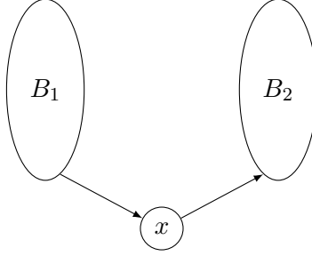
Figure 7: Structure of the tournament T_x^* used to show that ME violates \hat{\alpha}_\subseteq . Without alternative x , this is a minimal tournament T^* among those with multiple minimal extending sets (Theorem 2).
