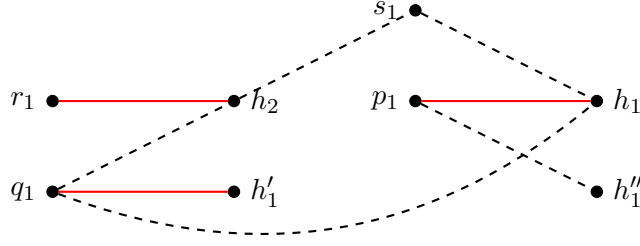
Figure 2: The edges of the matching N' are in red and the non-matching edges in G'_N are dashed. For simplicity, we have not included last resort neighbors here. Note that the edge (q_1, h_2) is a blocking edge to N' as both q_1 and h_2 prefer each other to their respective partners in N' , i.e., \text{wt}_N(q_1, h_2) = 2 and \text{wt}_N(e) = 0 for all other edges e in G'_N .
