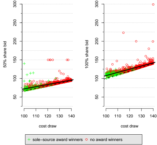
Figure 2: Bids of Sole-Source Award Winners for C = 0.67
