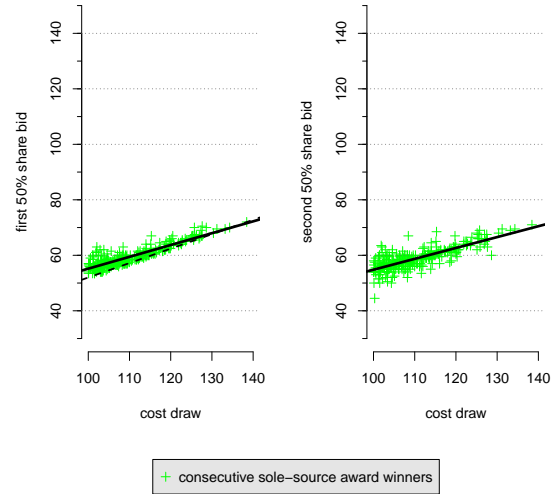
Figure 5: Bids of Consecutive Sole-Source-Award Winners for C = 0.52
