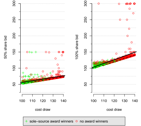
Figure 3: Bids of Sole-Source Award Winners for C = 0.52
