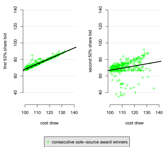
Figure 4: Bids of Consecutive Sole-Source-Award Winners for C = 0.67
